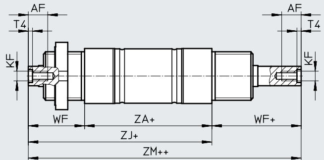
S2-K3 – Through piston rod, with female thread
