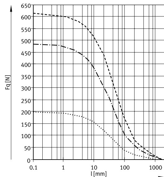
S2 – Through piston rod
