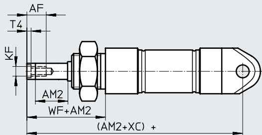
K3-K8 – Extended piston rod, with female thread
