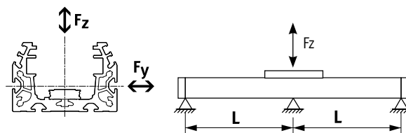
Force F_z
