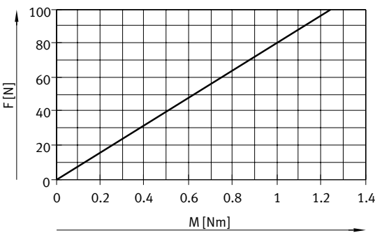
Feed force F_x as a function of input torque M
