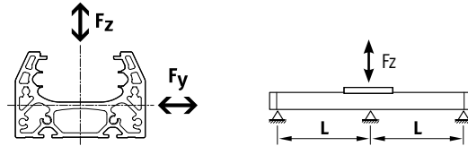
Force F_z
