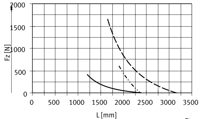
Force F_z
